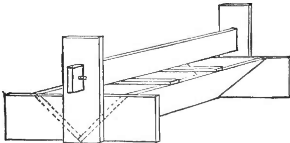
Fig. 19.—DOUBLE FEEDING TROUGH FOR PIGS.
