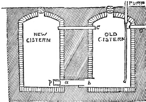
Fig. 142.—CONNECTING TWO CISTERNS.
