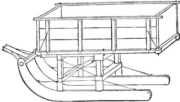
Fig. 46.—A SLED ARRANGED FOR DUMPING.
