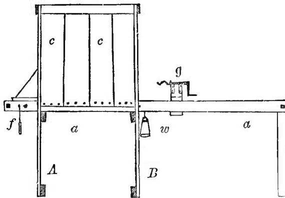
Fig. 167.—THE COMPLETE MACHINE (STRAW-TWISTER).
