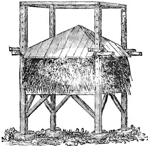
Fig. 155.—BARRACK WITH BOARD ROOF.
