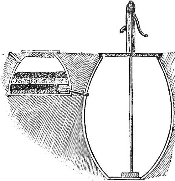
Fig. 144.—COMPLETE CISTERN AND FILTER.
