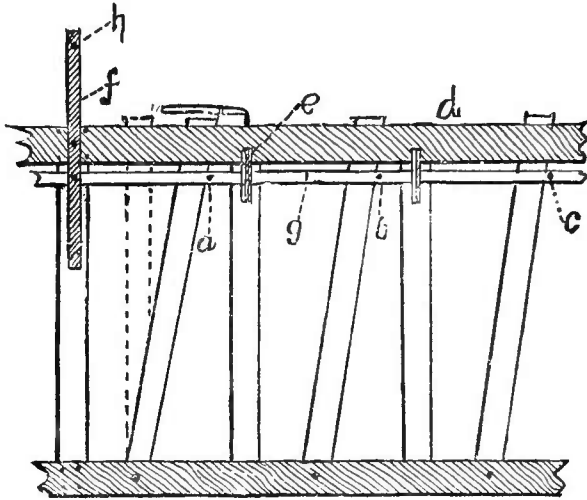
Fig. 9.—DEVICE FOR CLOSING CATTLE STANCHIONS.
