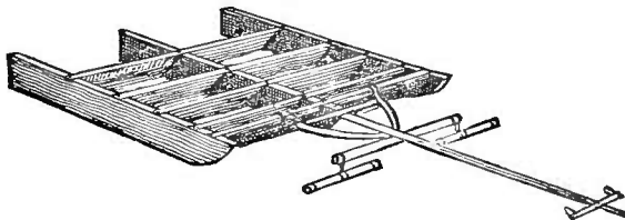
Fig. 61.—COMBINED MARKER AND CLOD CRUSHER.
