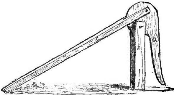
Fig. 40.—HOME-MADE WAGON-JACK.
