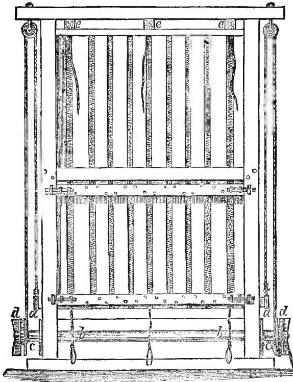
Fig. 159.—FRAME OF HAY PRESS.
