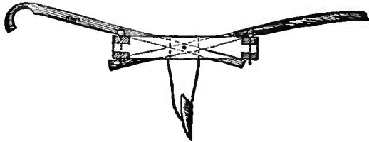
Fig. 57.—END VIEW OF LAND-MARKER.
