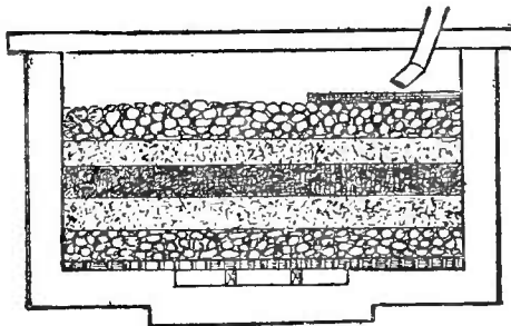
Fig. 145.—FILTER FOR A BARN CISTERN.
