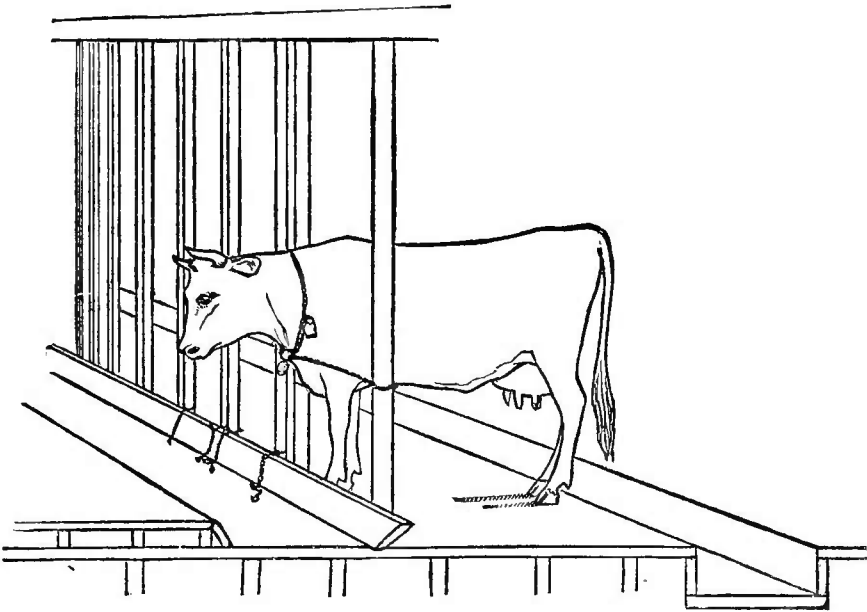
Fig. 10.—CHAIN CATTLE STANCHION.
