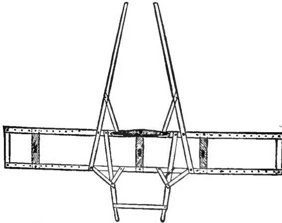
Fig. 56.—LAND-MARKER COMPLETE.
