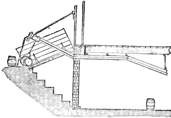
Fig. 183.—A CELLAR CARRIER.
