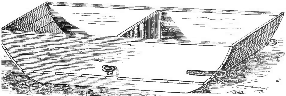
Fig. 189.—A BOAT FOR GETTING OUT MUCK.
