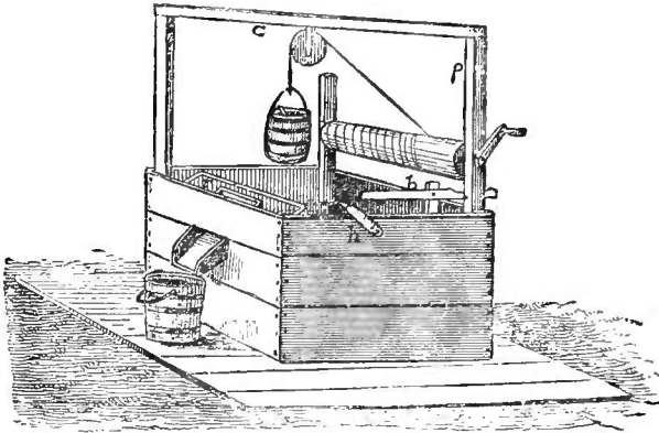
Fig. 122.—IMPROVED WINDLASS.
