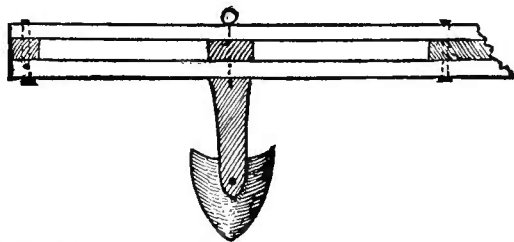
Fig. 58.—MOVABLE TOOTH OF LAND-MARKER.
