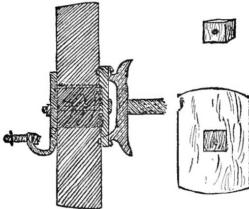
Fig. 73.—CENTER BLOCK.
