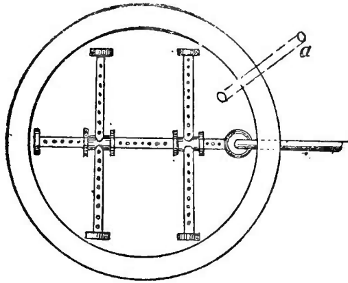
Fig. 147.—PIPES FOR HOUSE CISTERN.
