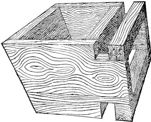
Fig. 6.—FENCE FEED BOX.
