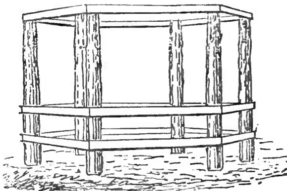
Fig. 158.—FRAME FOR STRAW OR HAY STACK.
