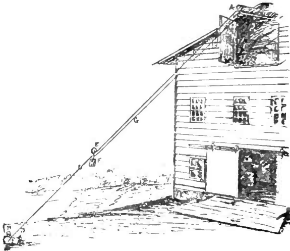
Fig. 154.—IMPROVED HAY-CARRIER.
