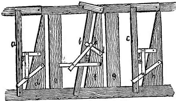
Fig. 8.—SELF-CLOSING CATTLE STANCHION.
