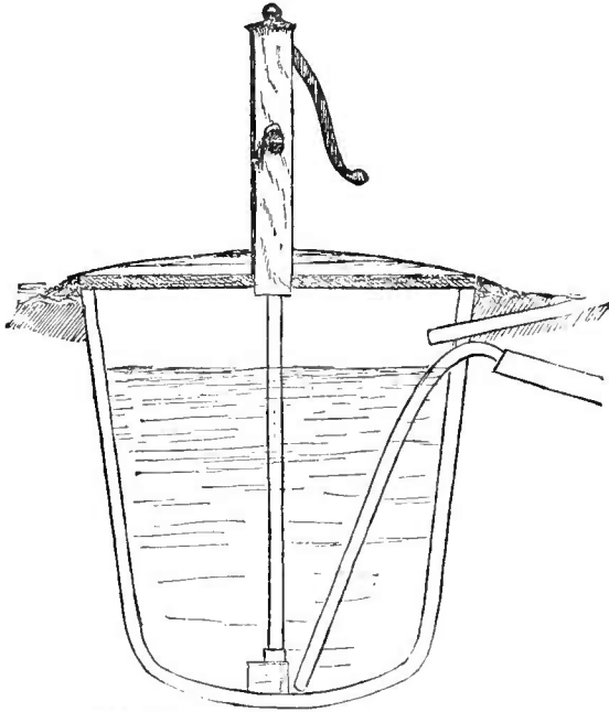
Fig. 137.—FROST-PROOF CISTERN.
