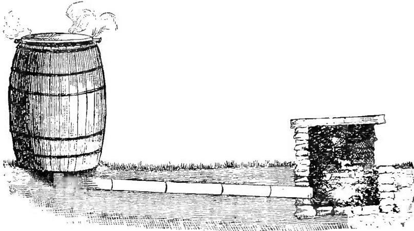
Fig. 237.—A BARREL SMOKE HOUSE.
