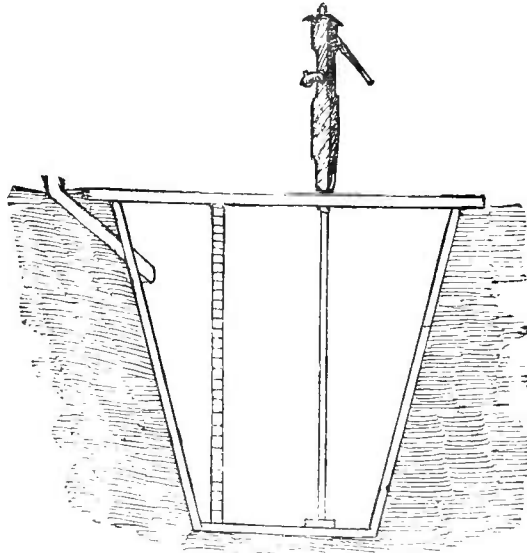
Fig. 143.—A COMPLETE CISTERN.
